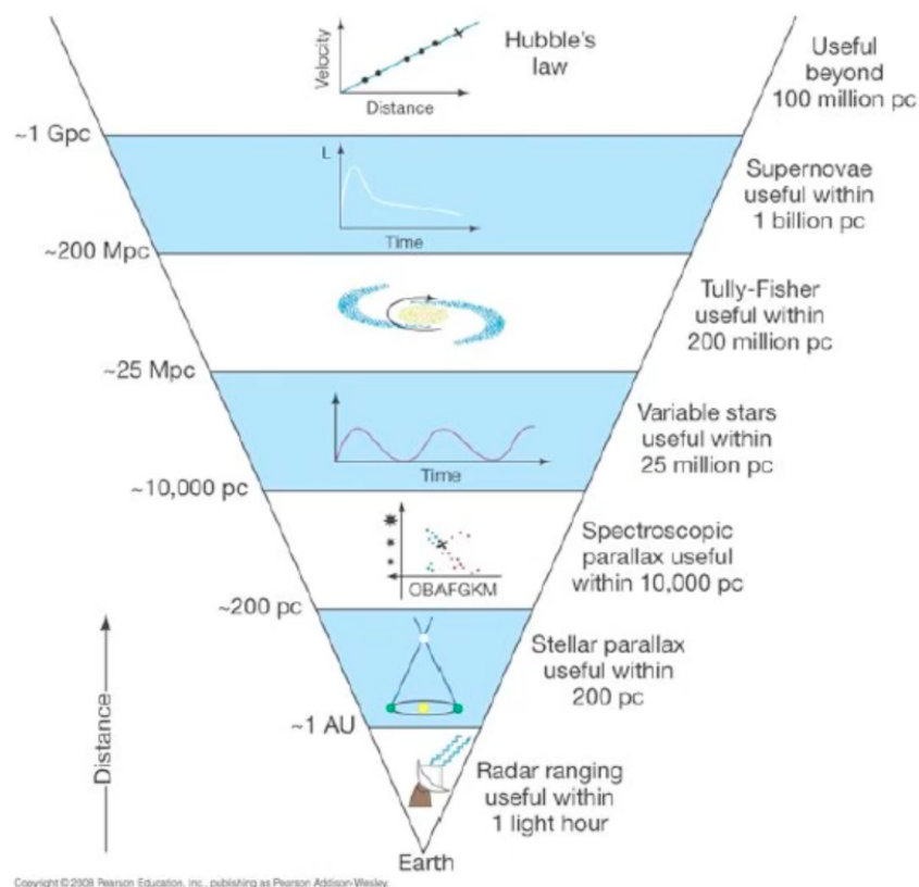
Figure 24.2: The Cosmic Distance Ladder
