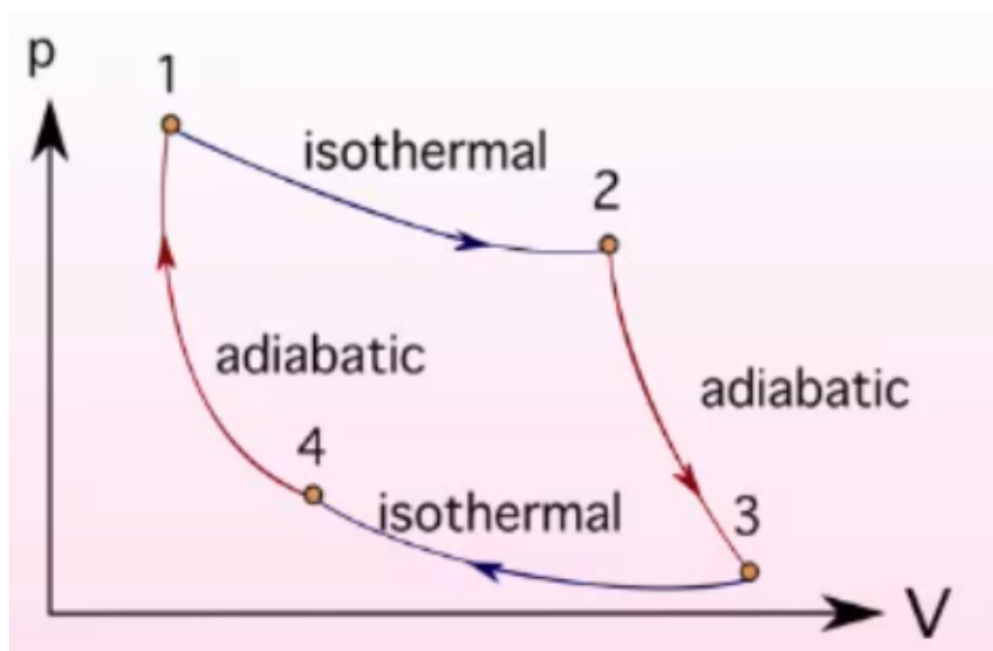
Figure 45.1: Differences in transitions on a PV Plot
